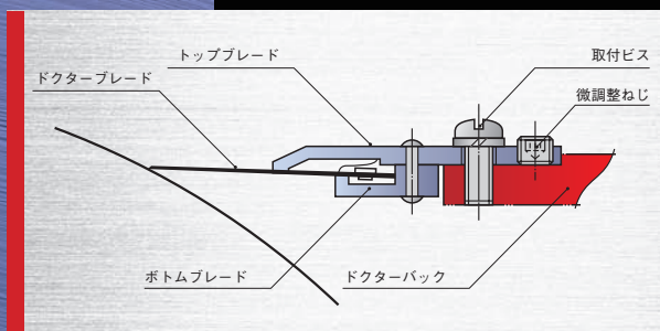
The sectional view of "KF-N type"
