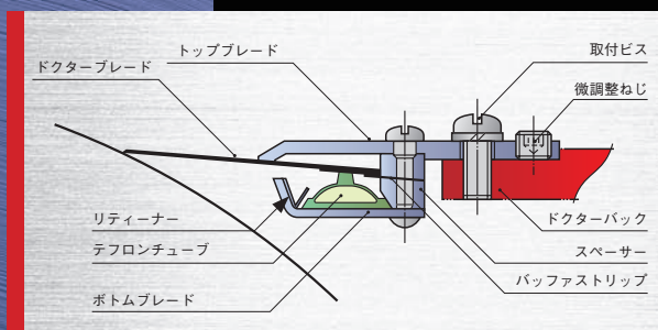
The sectional view of "CM type"
