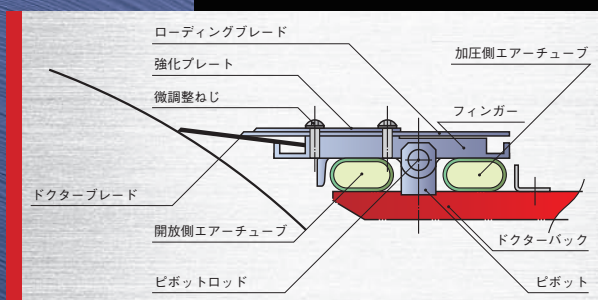
The sectional view of "DAC-A type"
